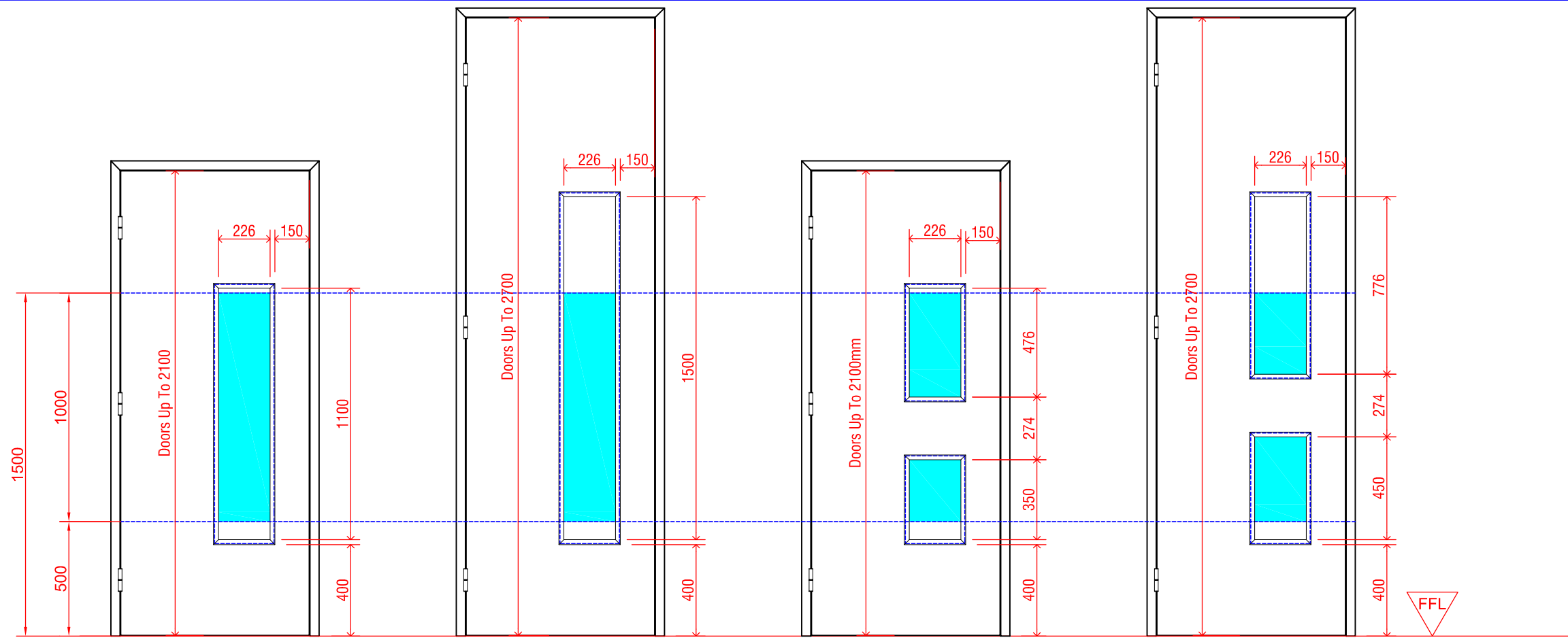
cgo = 226mm x 1100mm Aperture = 260mm x 1134 Glass Size = 254mm x 1128mm
